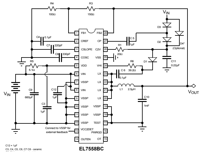
C12 = 1μF C3, C4, C5, C6, C7, C8 - ceramic C9, C11 - ceramic or tantalum C9 - Sprague 2930337X96R3 2x330μF C10 - Sprague 2950337X96R3 3x330μF L1 - Pulse Engineering, PE-63681 D1 - D4: BAT54S fast diode D4 Required for EL7558BCM only
