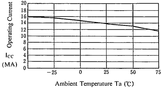
Operating Current vs. Ta (V + =5 V)
