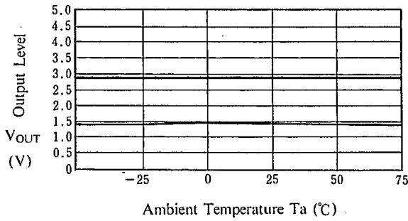
Output DC Level vs. Ta (V + =5 V)
