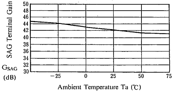
SAG Terminal Gain vs. Ta (V + =5 V)
