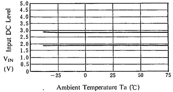
Input DC Level vs. Ta (V + =5 V)
