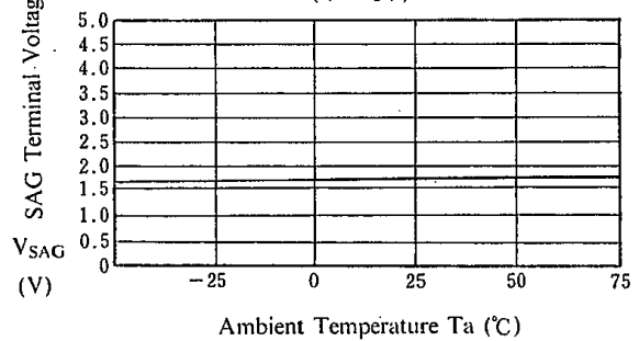
SAG Terminal Voltage vs. Ta (V + =5 V)
