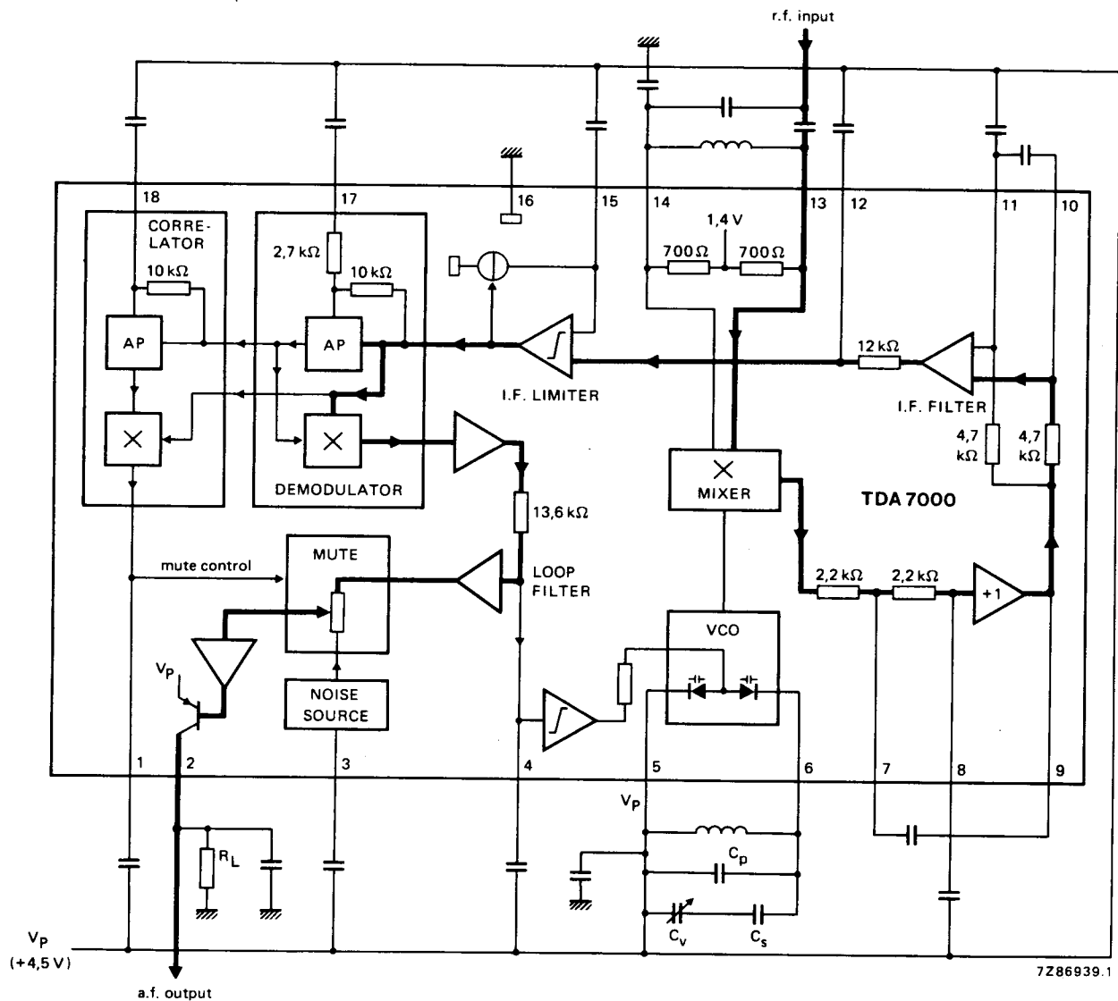
Fig. 1 Block diagram.
