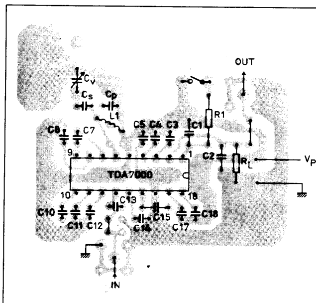
Fig. 6 Component side of printed-circuit board showing component layout used for the circuit of Fig. 4.
