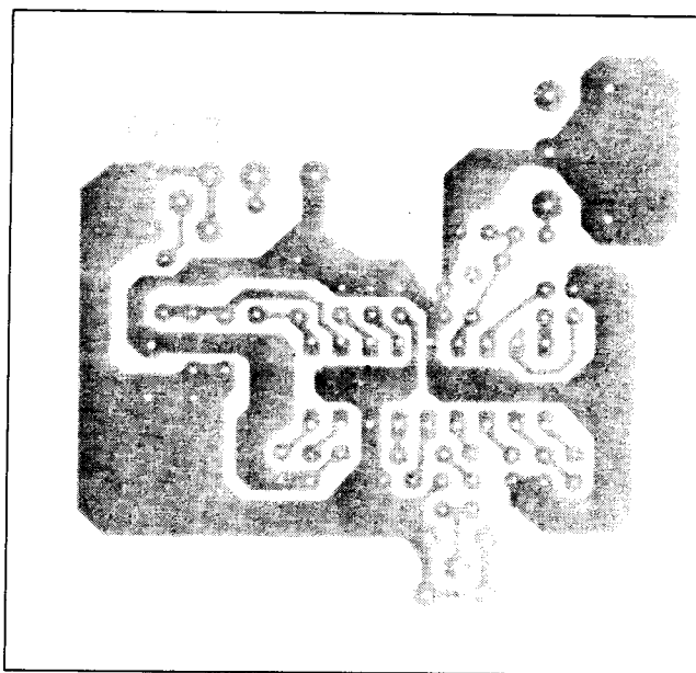
Fig. 5 Track side of printed-circuit board used for the circuit of Fig. 4.
