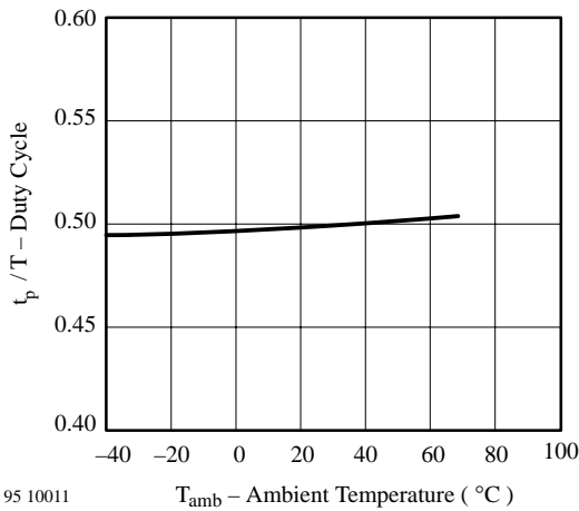
Figure 10 Duty Cycle vs. Ambient Temperature
