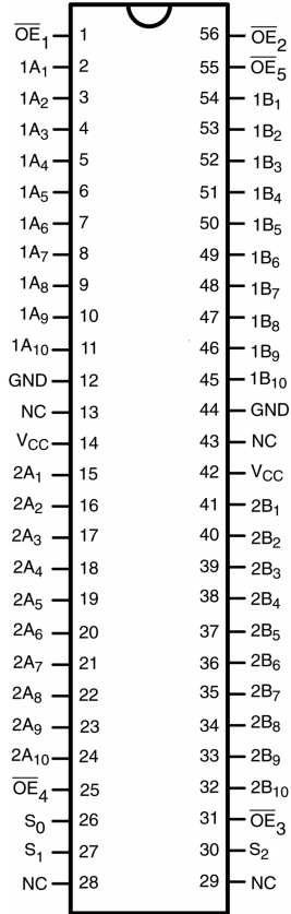
Pin Assignment for TSSOP
