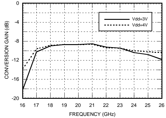
Conversion Gain, LO = -5 dBm Vdd = +4V
