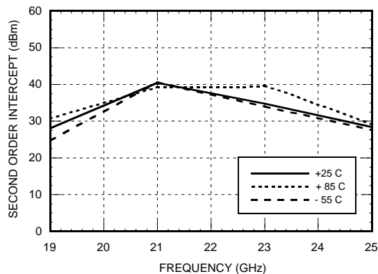
Input IP2 vs. Temperature @ LO = -5 dBm, Vdd = +3V *
