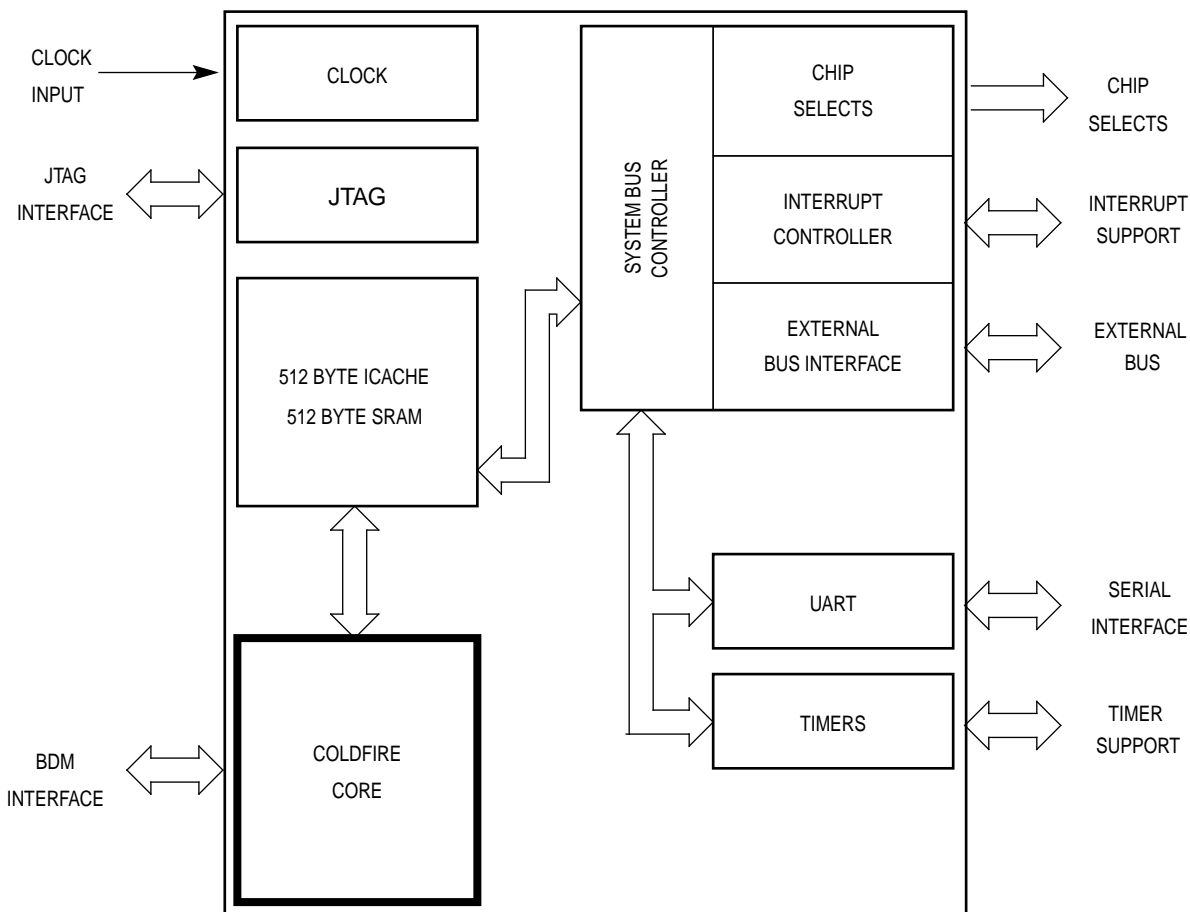
Figure 1. MCF5204 Block Diagram
