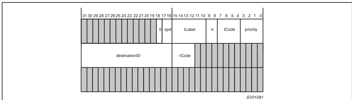
Figure 15. Quadlet/Block Write Response Packet Transmit Format
