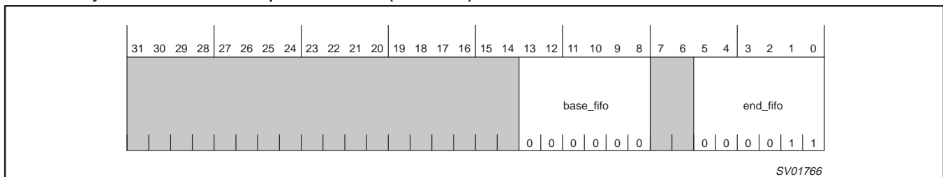
Figure 34. Reset situation of size programmable FIFOs
