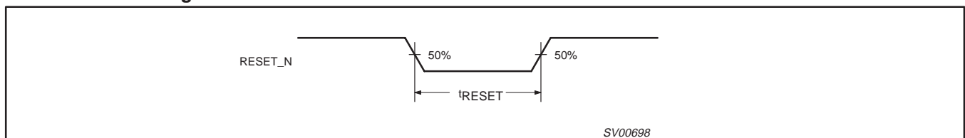
Figure 43. RESET_N Waveform
