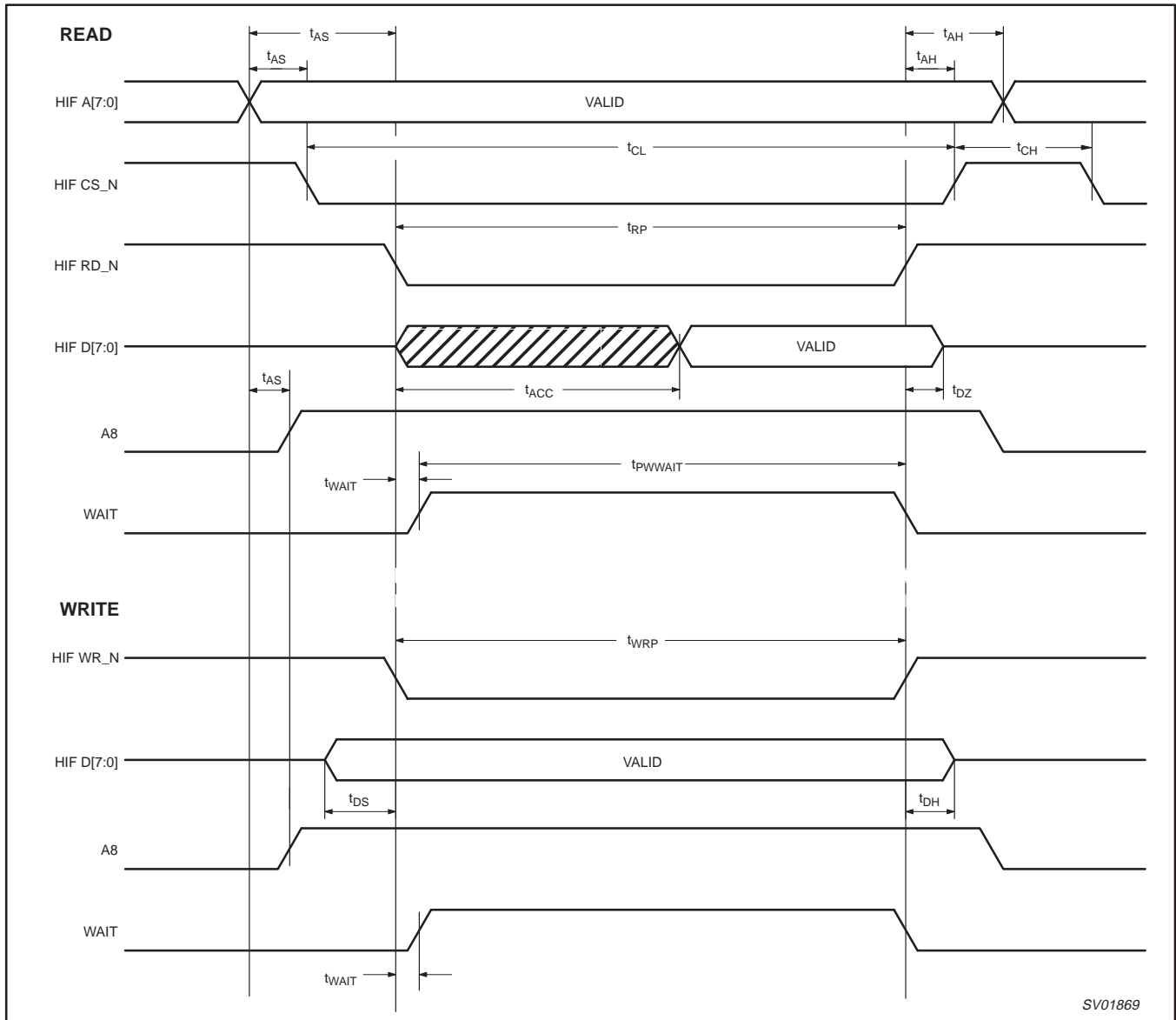
Figure 40. Host Interface Timing Waveforms
