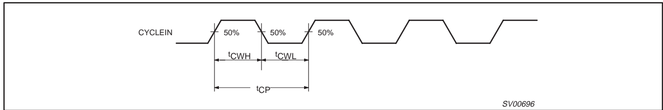
Figure 41. CYCLEIN Waveform
