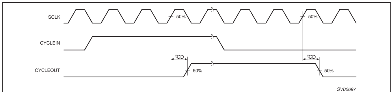
Figure 42. CYCLEOUT Waveforms
