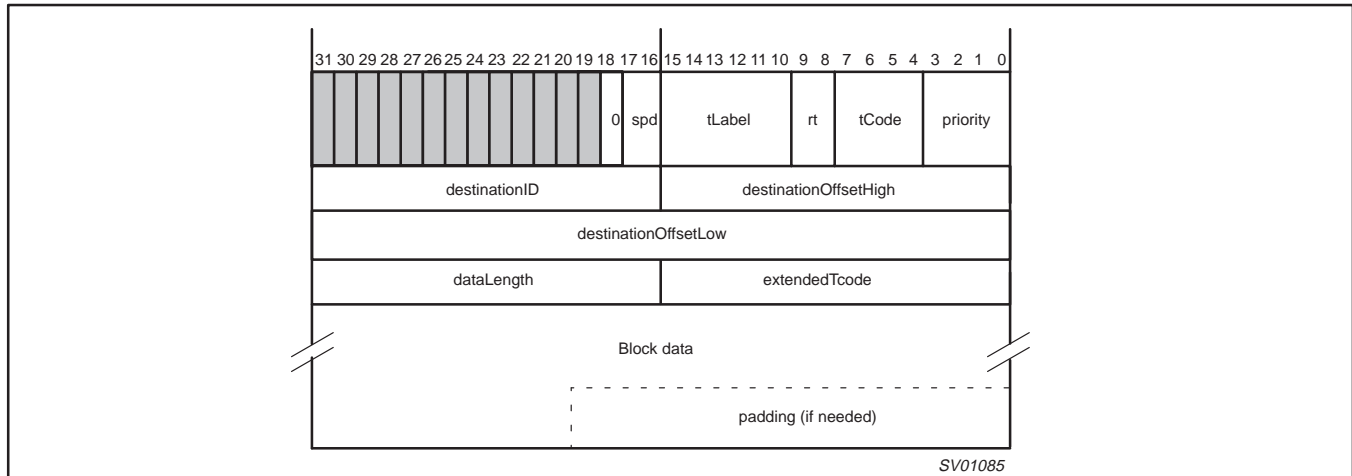
Figure 19. Block Packet Transmit Format
