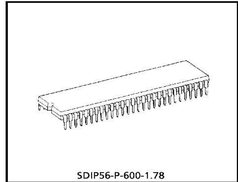
SDIP56-P-600-1.78
