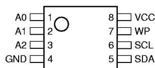
8-Pin MSOP
