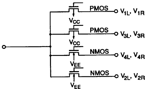
Output Terminal
