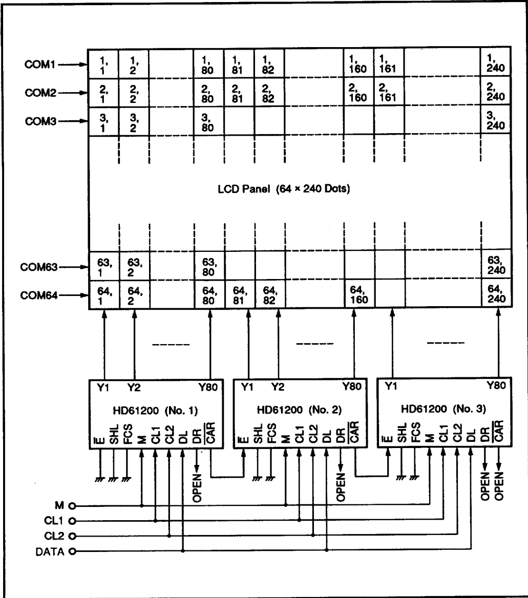
Figure 1 LCD Driver with 64 x 240 Dots
