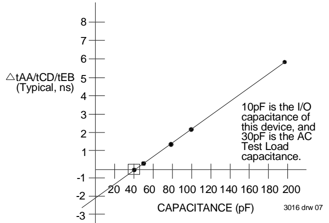
Figure 3. Lumped Capacitance Load Typical Derating Curve
