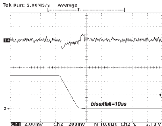
V_{IN} = 4.75 \text{ to } 5.25V, I_{OUT} = 0.1A, C_o = 10\mu F \text{ (ESR}=1\Omega \text{ at } 1KHz)
