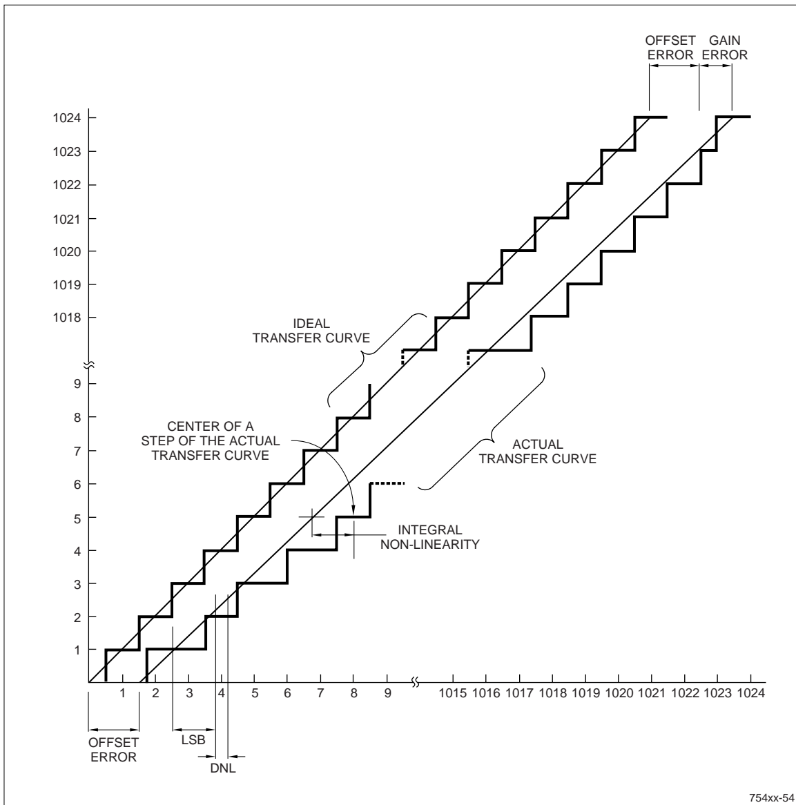
Figure 10. ADC Transfer Characteristics
