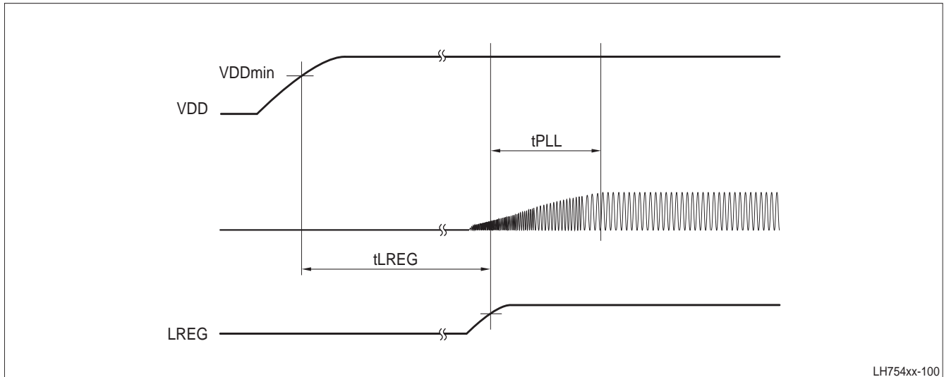
Figure 11. Power-up Stabilization
