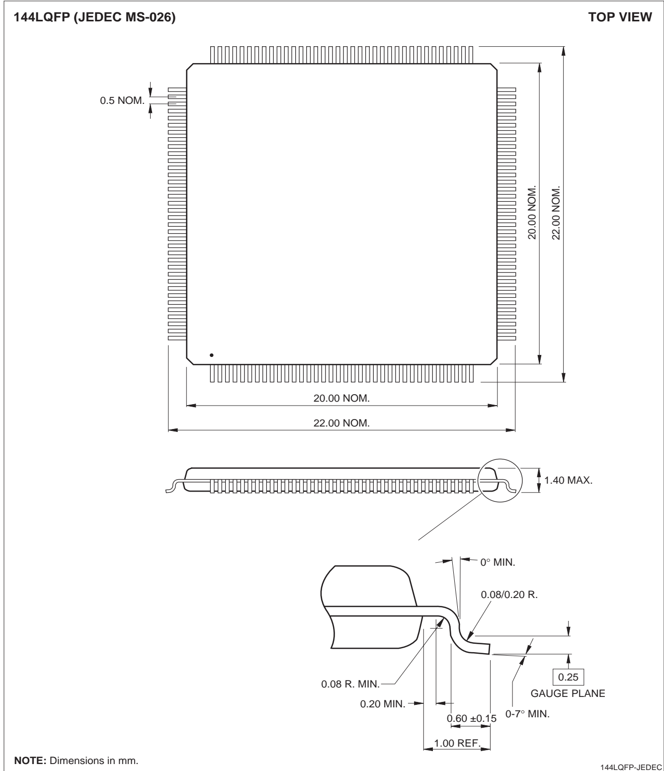
Figure 17. 144-pin LQFP
