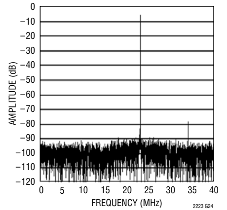
LTC2222: 8192 Point FFT, f_{IN} = 500\text{MHz} , -6dB, 1V Range
