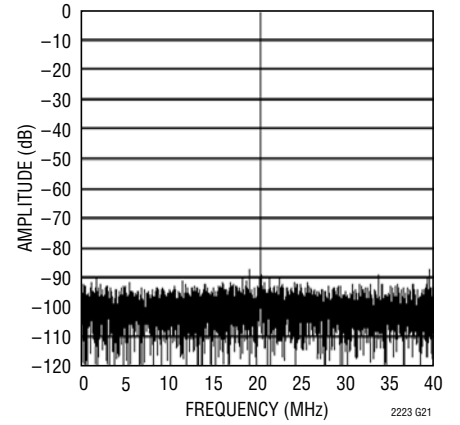
LTC2222: 8192 Point FFT, f_{IN} = 140\text{MHz} , -1dB, 1V Range
