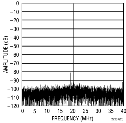
LTC2222: 8192 Point FFT, f_{IN} = 140\text{MHz} , -1dB, 2V Range
