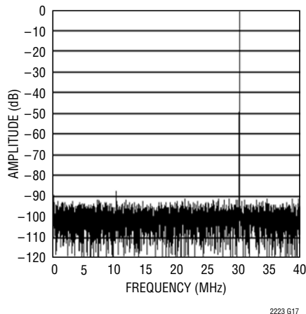
LTC2223: 8192 Point FFT, f_{IN} = 30\text{MHz} , -1\text{dB} , 1V Range
