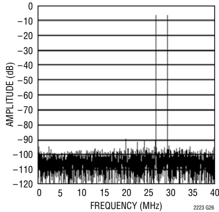
LTC2222: 8192 Point 2-Tone FFT, f_{IN} = 138\text{MHz} and 140\text{MHz} , -7dB Each, 1V Range
