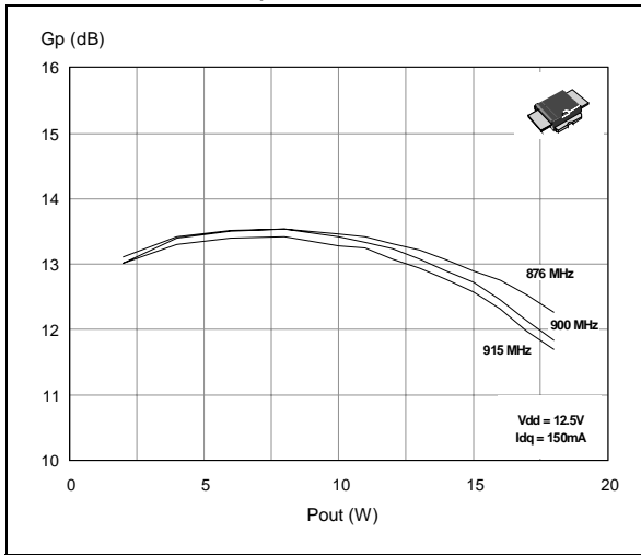
Power Gain vs. Output Power PD55015S
