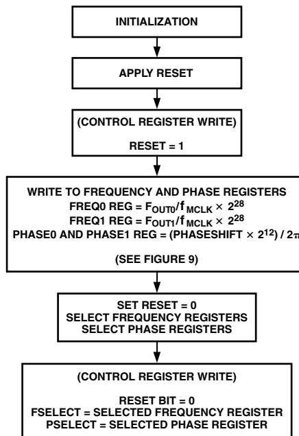
Figure 8. Initialization
