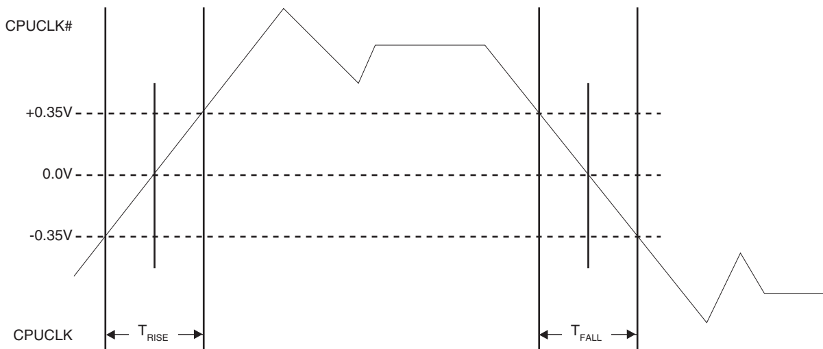
Figure 2 - 0.7V Differential TRise and TFall Measurement Points
