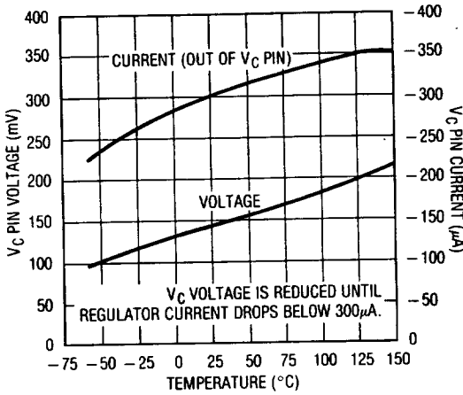
Shutdown Thresholds
