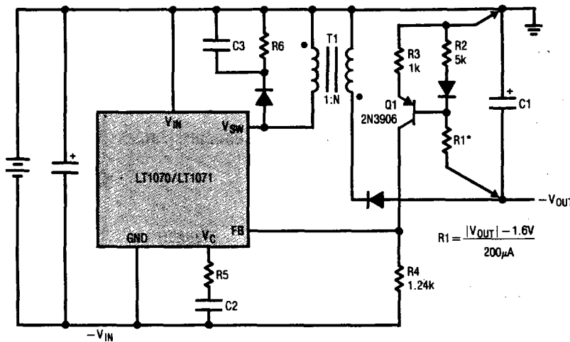
Forward Converter
