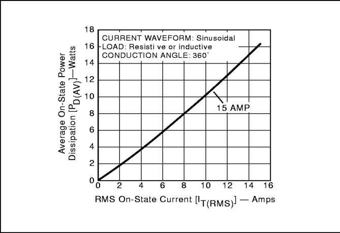
Figure 4.14 Power Dissipation (Typical) vs On-State Current (15 Amp Devices)
