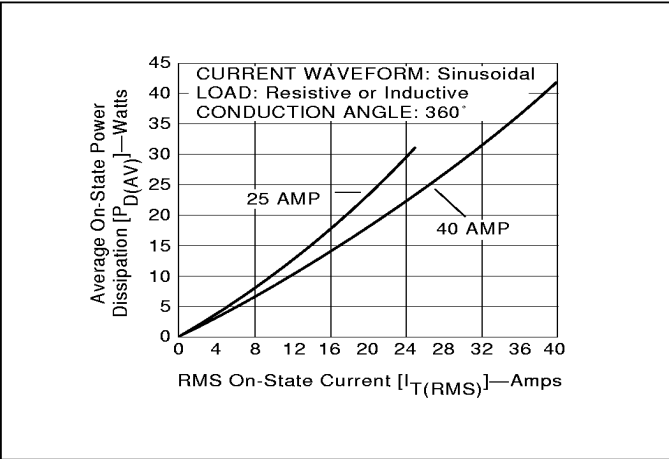
Figure 4.15 Power Dissipation (Typical) vs On-State Current (25 and 40 Amp Devices)
