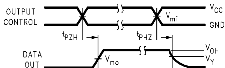
FIGURE 3. 3-STATE High Enable and Disable Times for Low Voltage Logic
