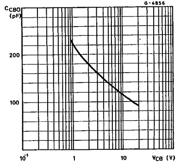
Collector-base Capacitance (PNP types).
