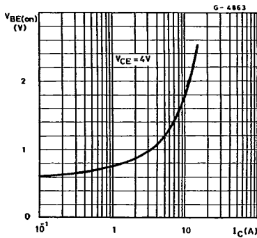
DC Transconductance (NPN types).
