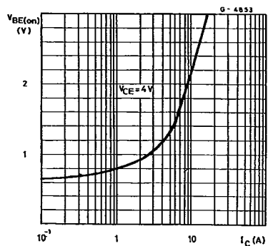
DC Transconductance (PNP types).
