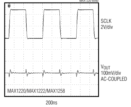
DAC DIGITAL FEEDTHROUGH RLOAD = 10kΩ, CLOAD = 100pF, CS = HIGH, DIN = LOW
