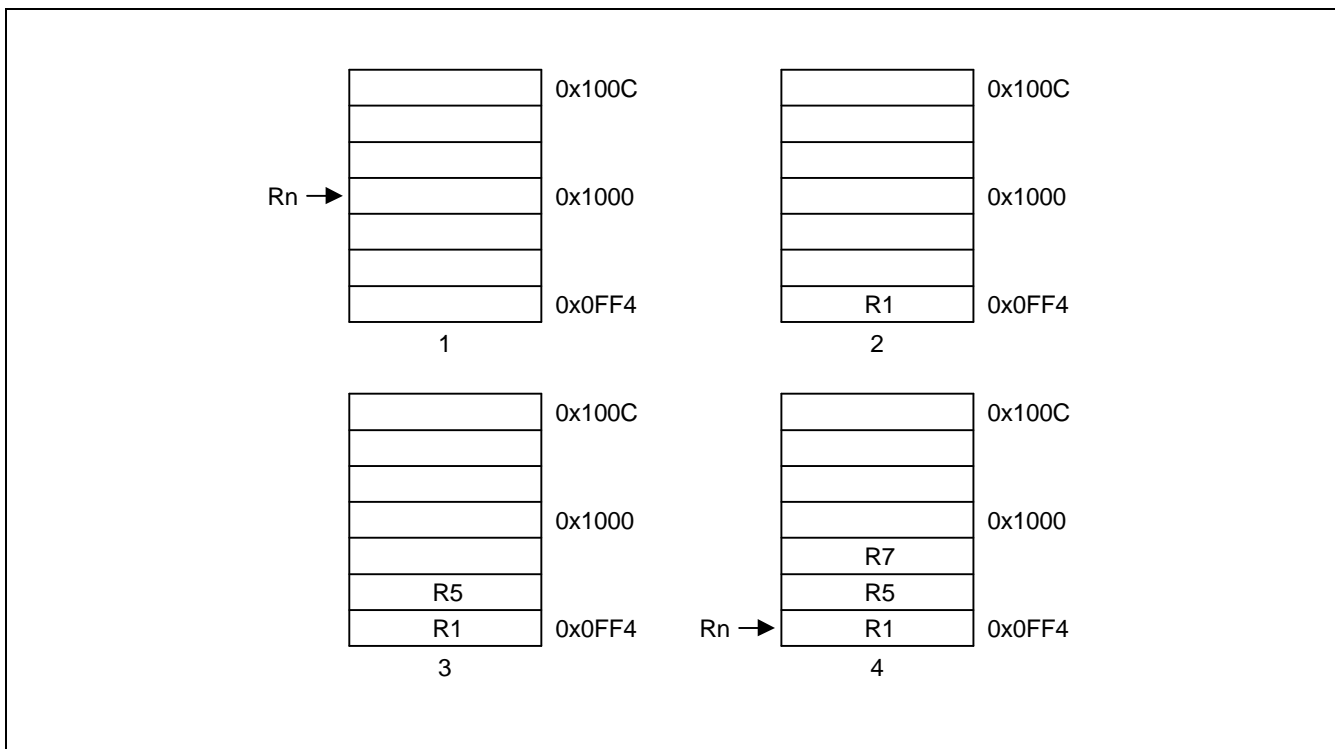
Figure 3-22. Pre-Decrement Addressing
