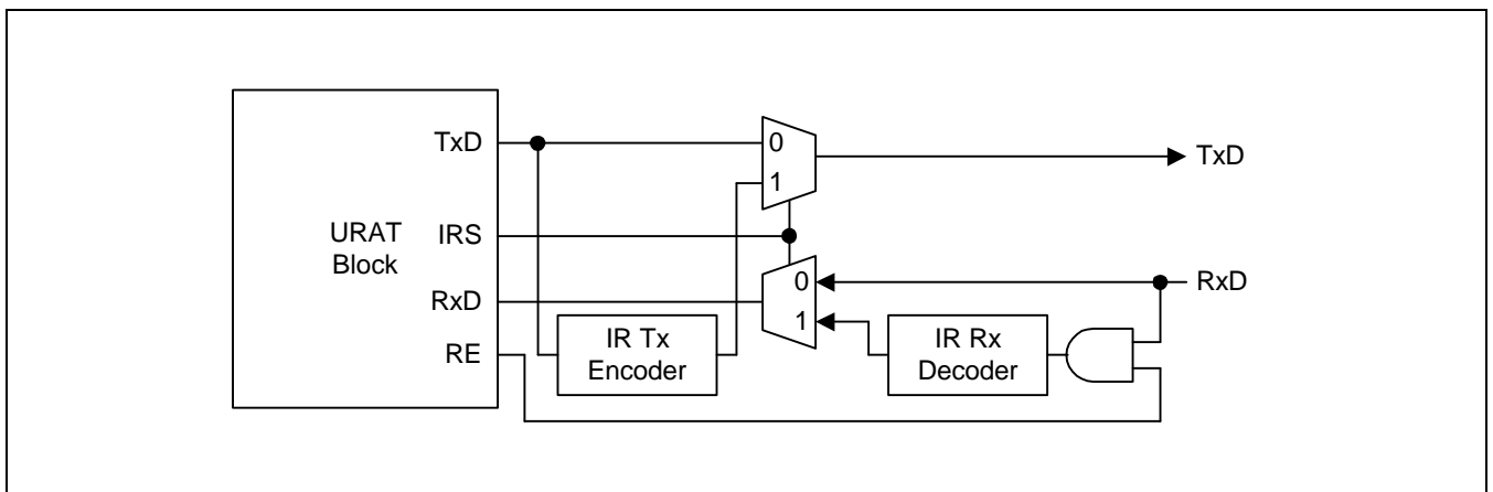
Figure 7-2. Infra-red Mode
