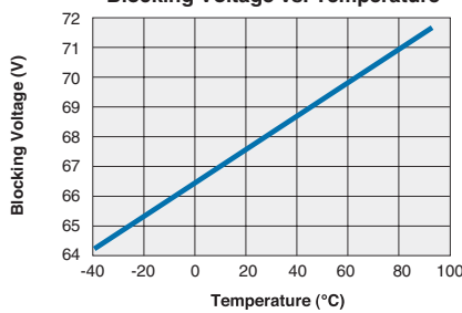
CPC1906Y Blocking Voltage vs. Temperature
