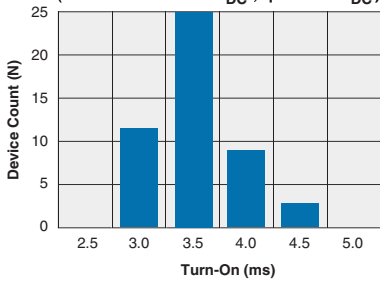
CPC1906Y Typical Turn-On Time (N=50 Ambient Temperature = 25°C) (Load Current = 1\text{A}_{DC} ; I_F = 10\text{mA}_{DC} )
