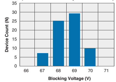
CPC1906Y Typical Blocking Voltage Distribution (N=50 Ambient Temperature = 25°C)
