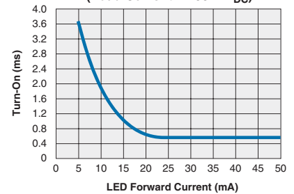
CPC1906Y Typical Turn-On vs. LED Forward Current (Load Current = 100\text{mA}_{DC} )
