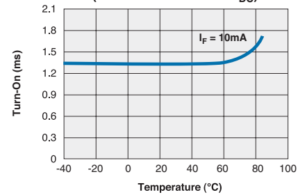
CPC1906Y Typical Turn-On vs. Temperature (Load Current = 100\text{mA}_{DC} )
