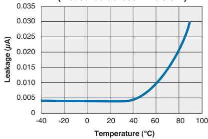
CPC1906Y Typical Leakage vs. Temperature at Maximum Rated Voltage (Measured across Pins 3 & 4)
