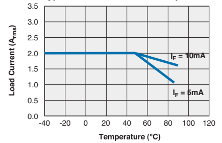
CPC1906Y Typical Load Current vs. Temperature
