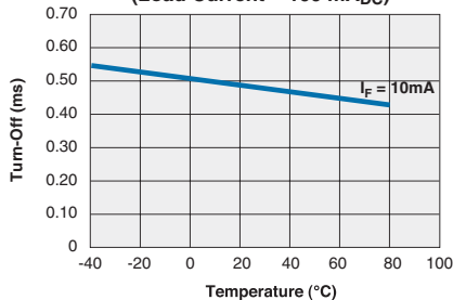
CPC1906Y Typical Turn-Off vs. Temperature (Load Current = 100\text{mA}_{DC} )
