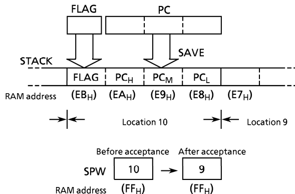
(b) At acceptance of an interrupt
