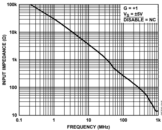
Figure 31. Input Impedance vs. Frequency
