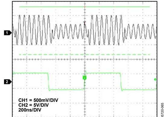
Figure 52. ADA4899-1 2:1 Mux Transient Response
