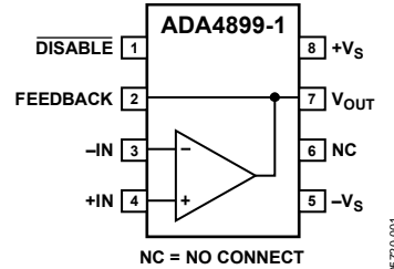
Figure 1. 8-Lead LFCSP_VD (CP-8)
