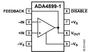
Figure 2. 8-Lead SOIC_N_EP (RD-8)
