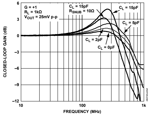
Figure 9. Small Signal Frequency Response for Capacitive Loads
