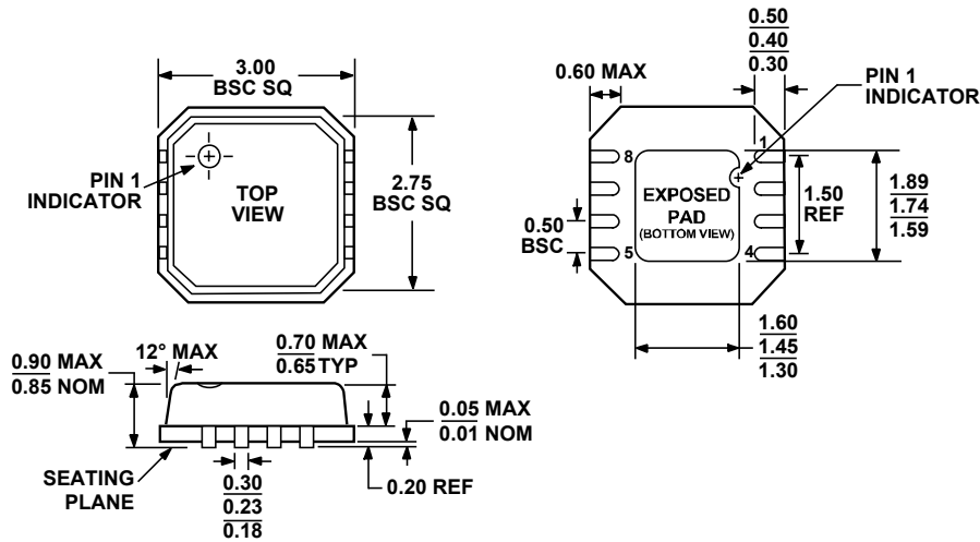
Figure 54. 8-Lead Lead Frame Chip Scale Package [LFCSP_VD]
