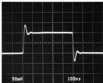
Small-Signal Transient (G = 1)
