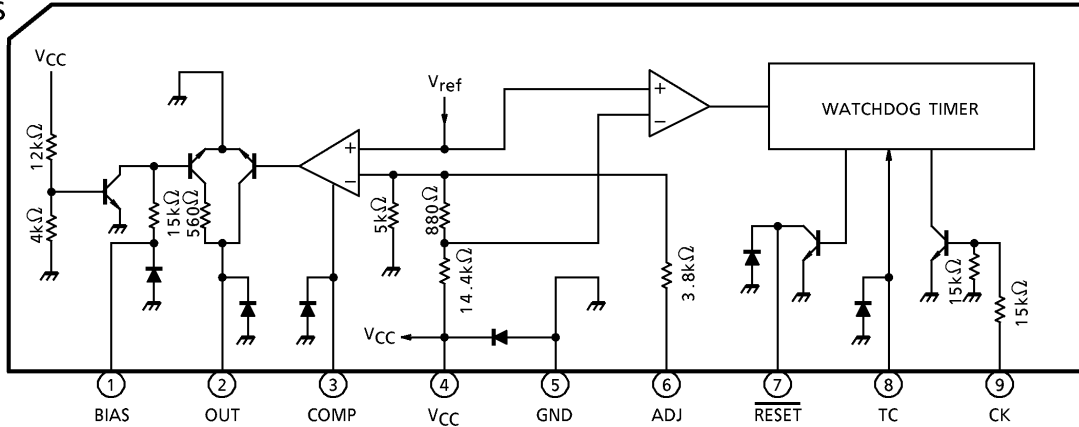
TA8000S
