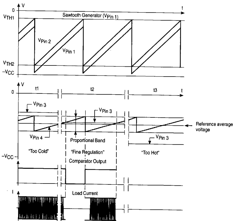
Figure 2. Sawtooth Generator and Proportional Band
