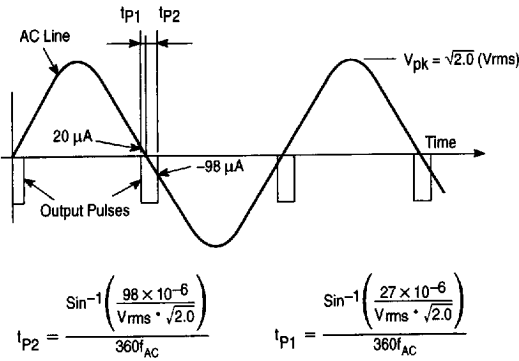
Figure 3. Output Pulse Width Definitions
