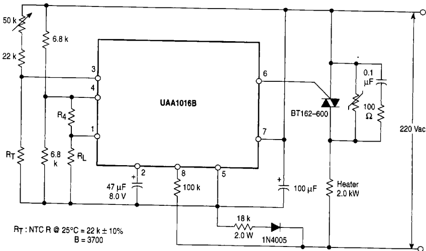
Figure 9. Application Circuit—Electric Radiator with Proportional Band Thermostat (Proportional Band 1°C at 25°C)
