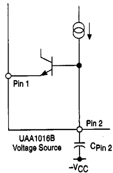
Figure 6. Pin 1 Internal Network
