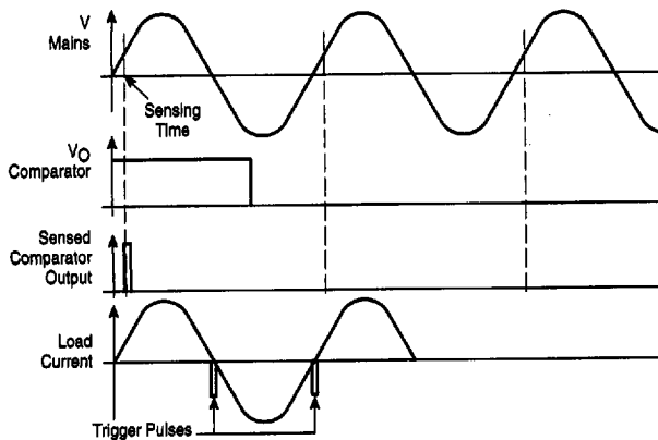
Figure 7. Trigger Pulse Generation
