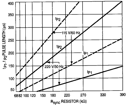
Figure 4. Typical Output Pulse Length versus Synchronization Resistor
