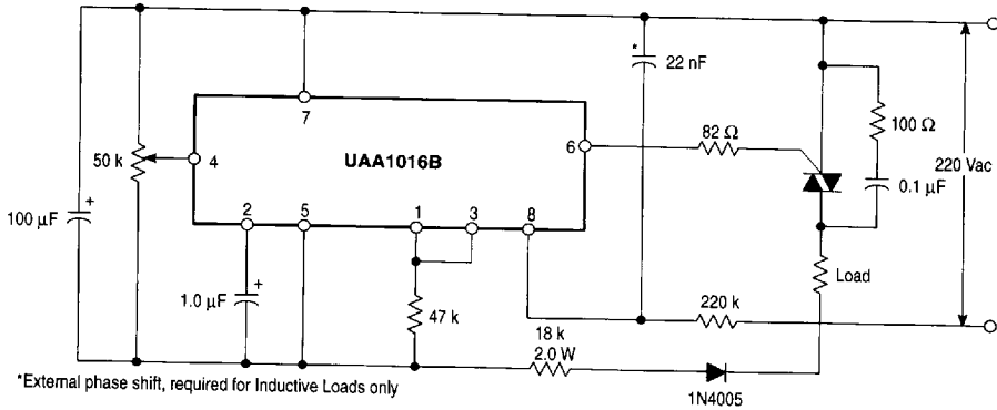
Figure 8. Electronic Rheostat
