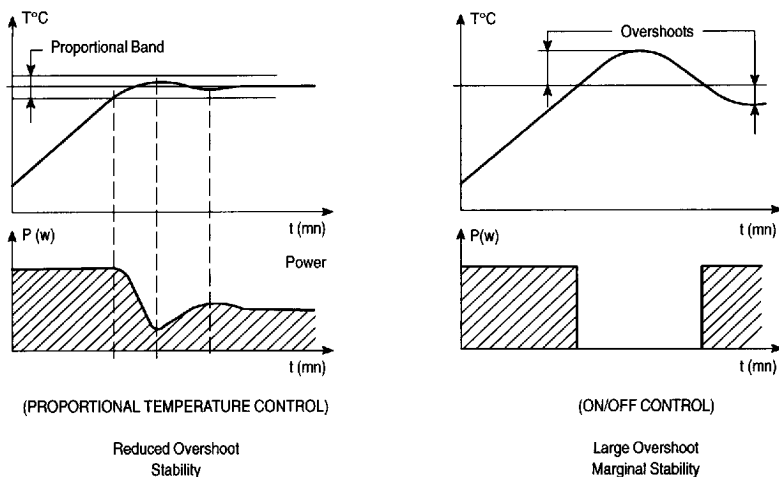
Figure 1. Proportional Temperature Control versus On/Off Control
