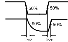
Fig. 5 Propagation delay time (CONT→OUT)
