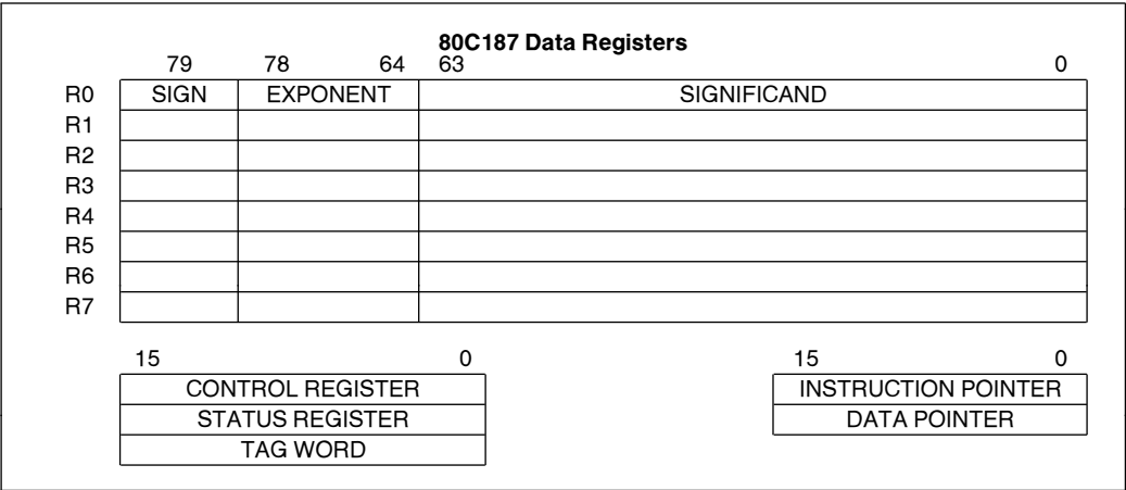
Figure 2. Register Set
