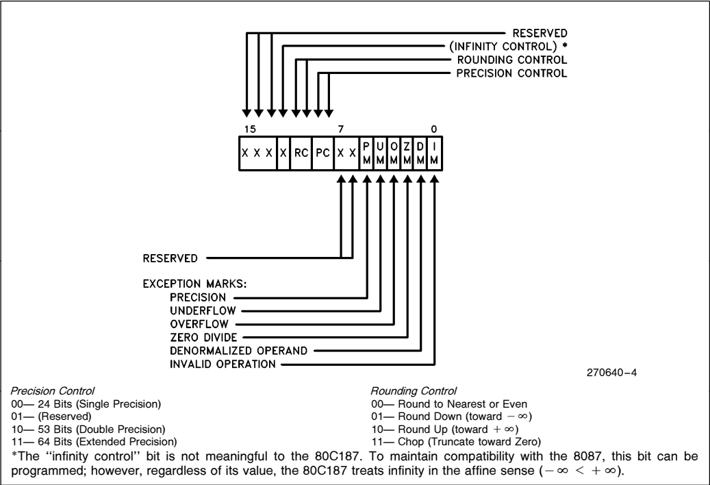
Figure 5. Control Word
