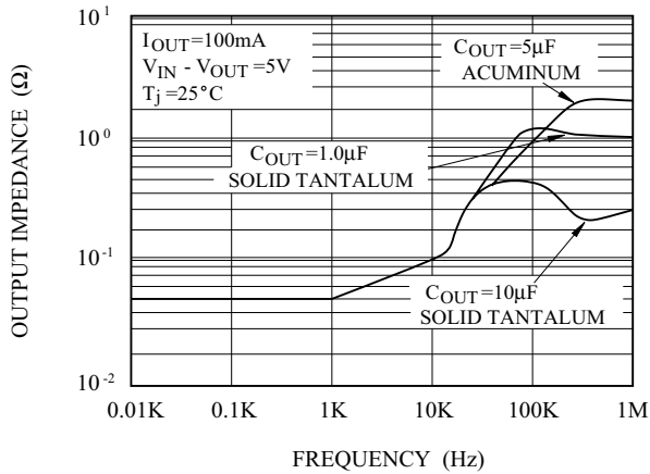
OUTPUT IMPEDANCE
