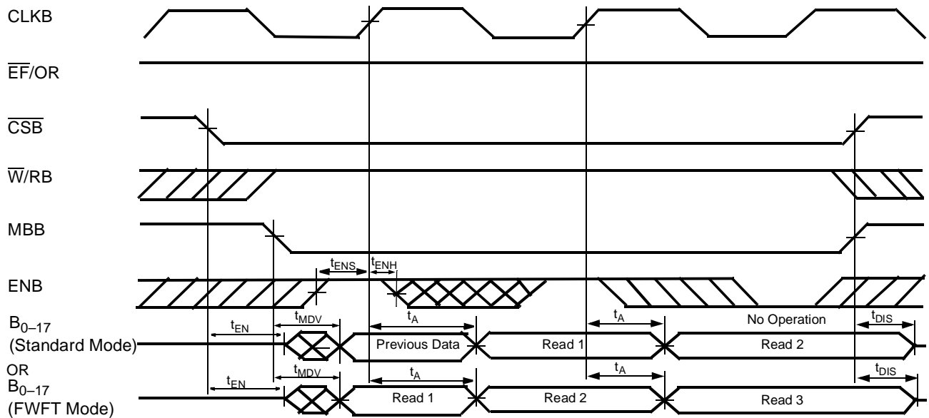
Port B Word Read Cycle Timing for FIFO (CY Standard and FWFT Modes) [19]
