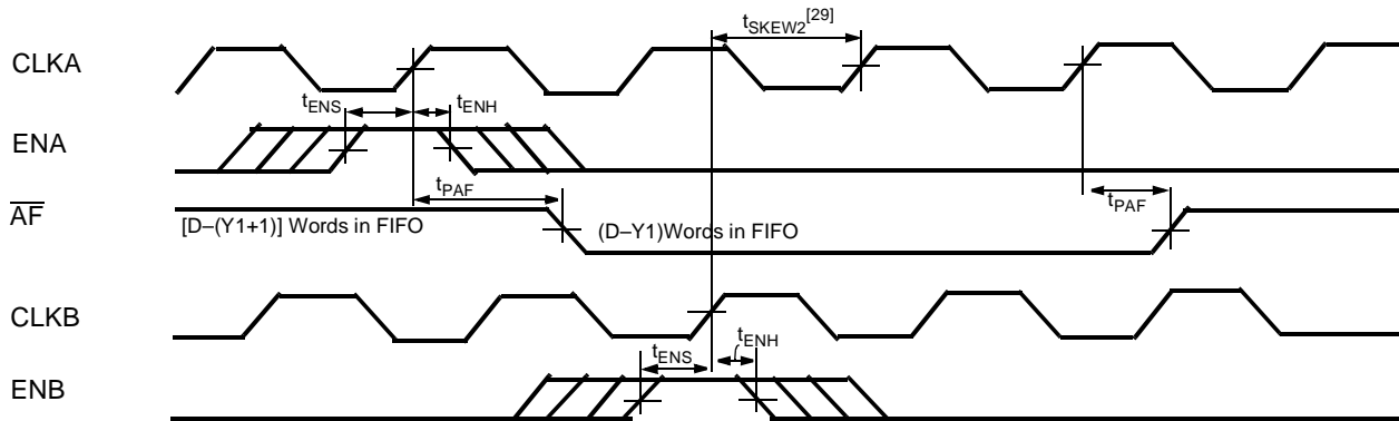
Timing for \overline{AF} when FIFO is Almost Full (CY Standard and FWFT Modes) [26, 27, 28]
