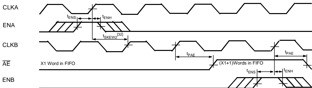
Timing for \overline{AE} when FIFO is Almost Empty (CY Standard and FWFT Modes) [30, 31]
