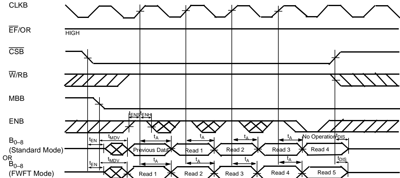
Port B Byte Read Cycle Timing for FIFO (CY Standard and FWFT Modes) [18]
