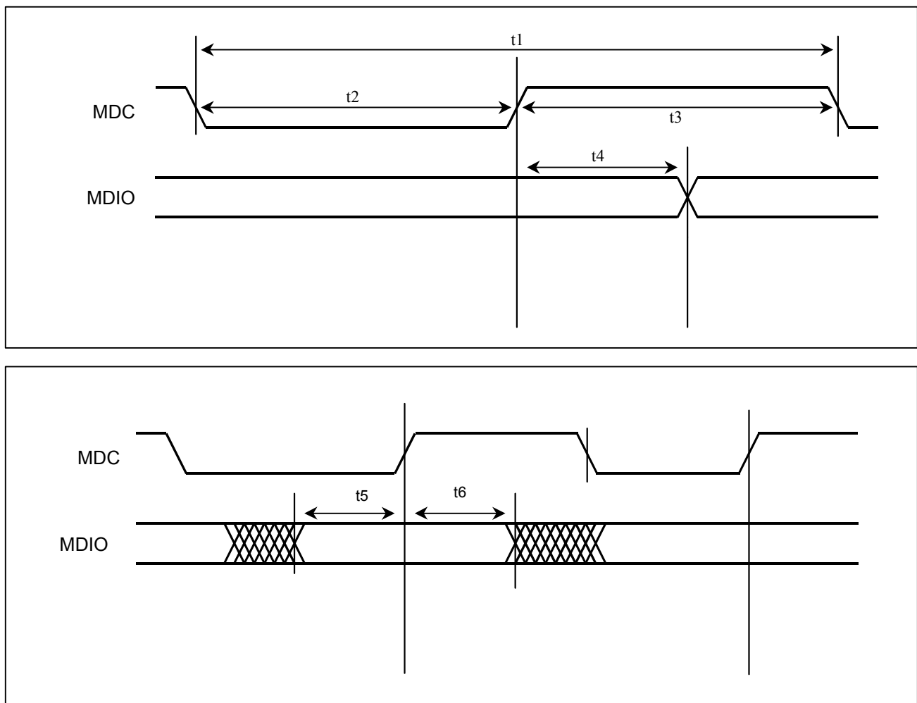
Figure 11-5 MDIO Timing
