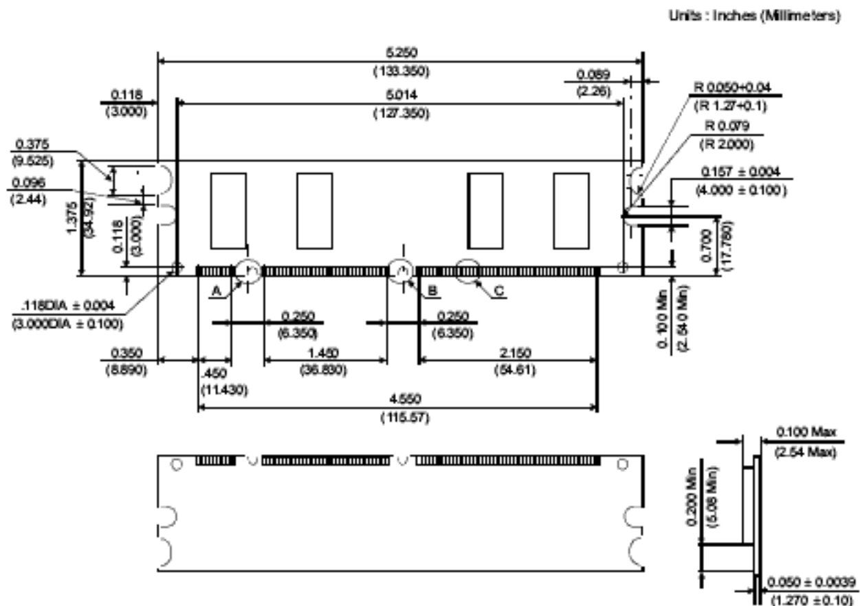
Figure 1: KVR133X64C2/128 168-Pin DIMM
