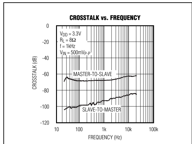
Figure 9. Master-Slave Crosstalk
