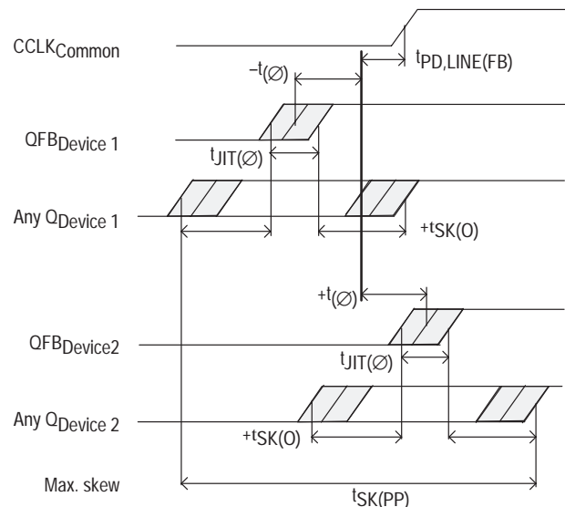
Figure 4. MPC9608 max. device-to-device skew
