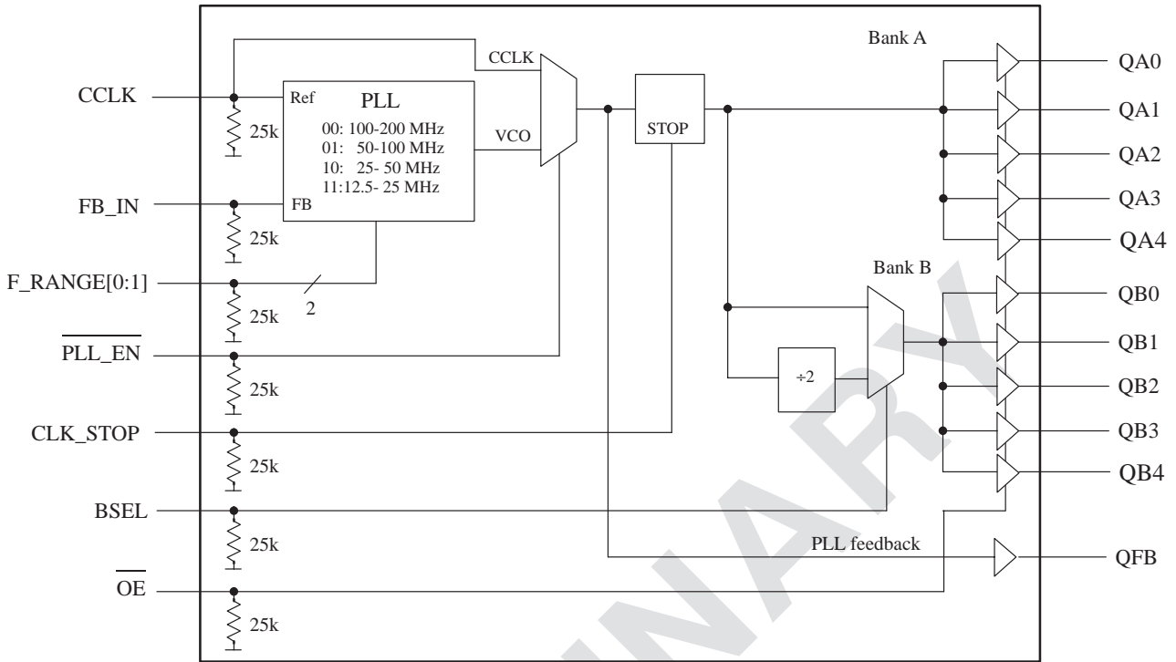
Figure 1. MPC9608 Logic Diagram
