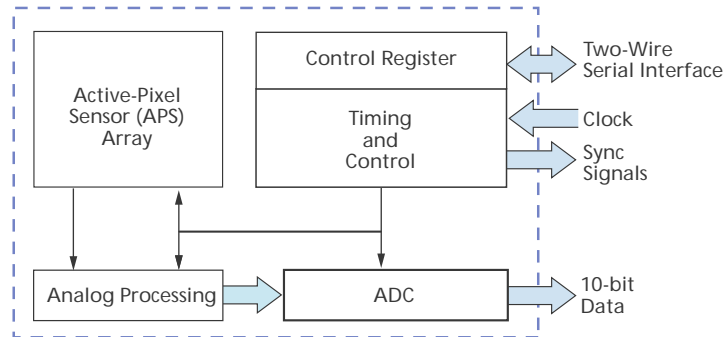
Figure 1: Block Diagram
