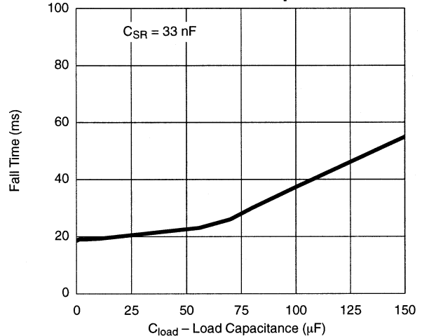
Switch 4 Fall Time vs. Load Capacitance
