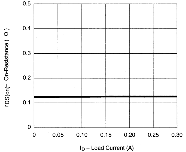
Switch 4—On-Resistance vs. Load Current
