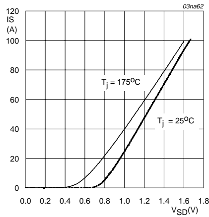
Fig 15. Reverse diode current; typical values.
