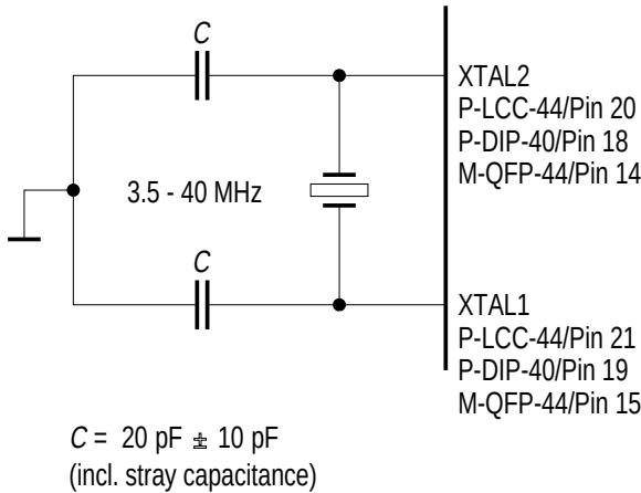
Crystal Oscillator Mode
