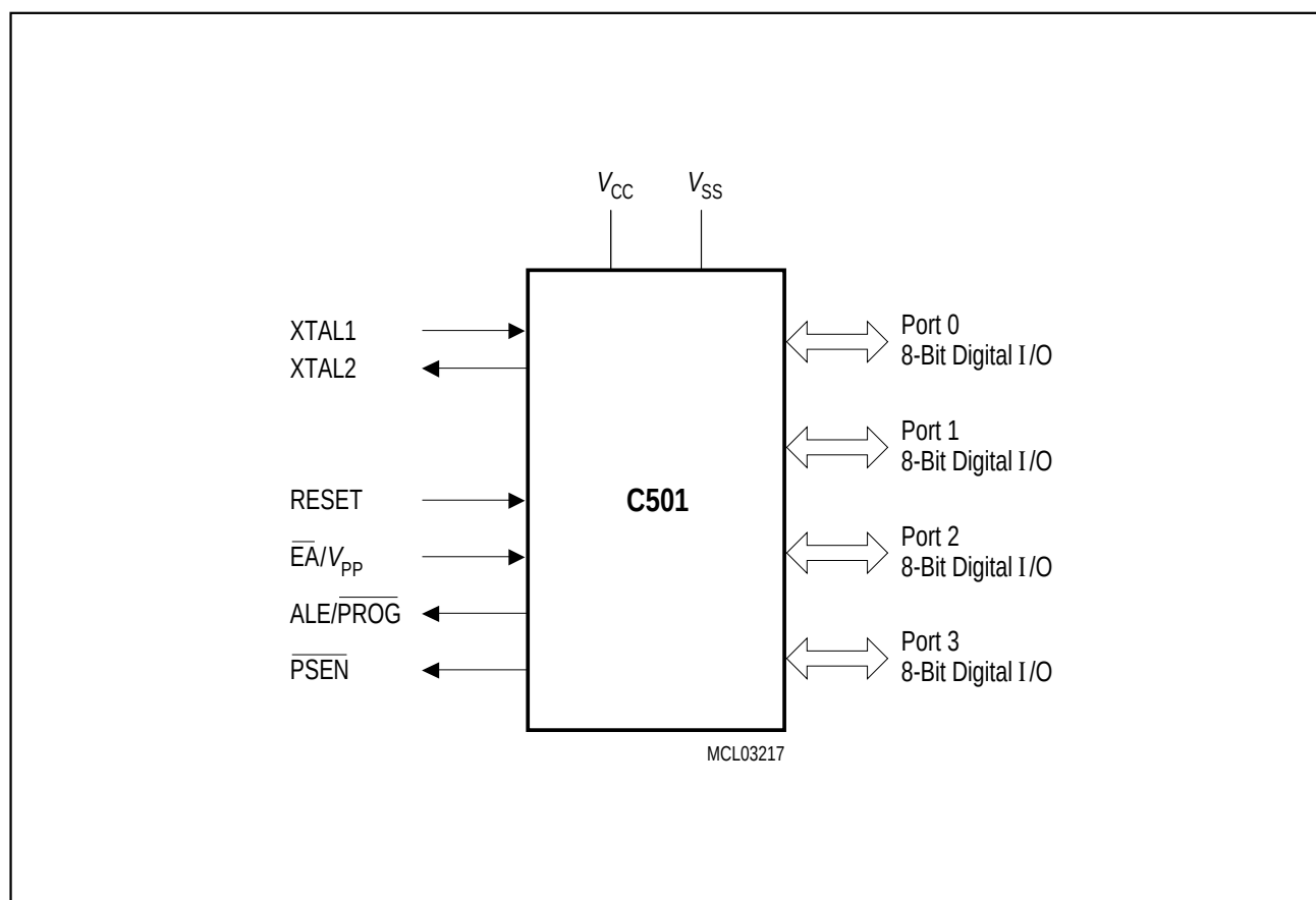
Figure 1-2 Logic Symbol
