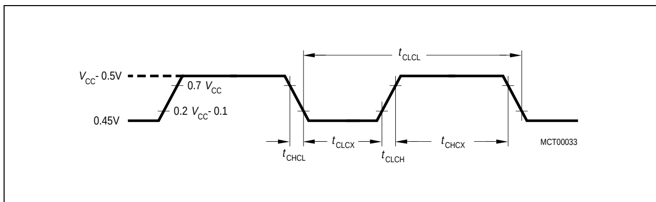
External Clock Drive at XTAL2
