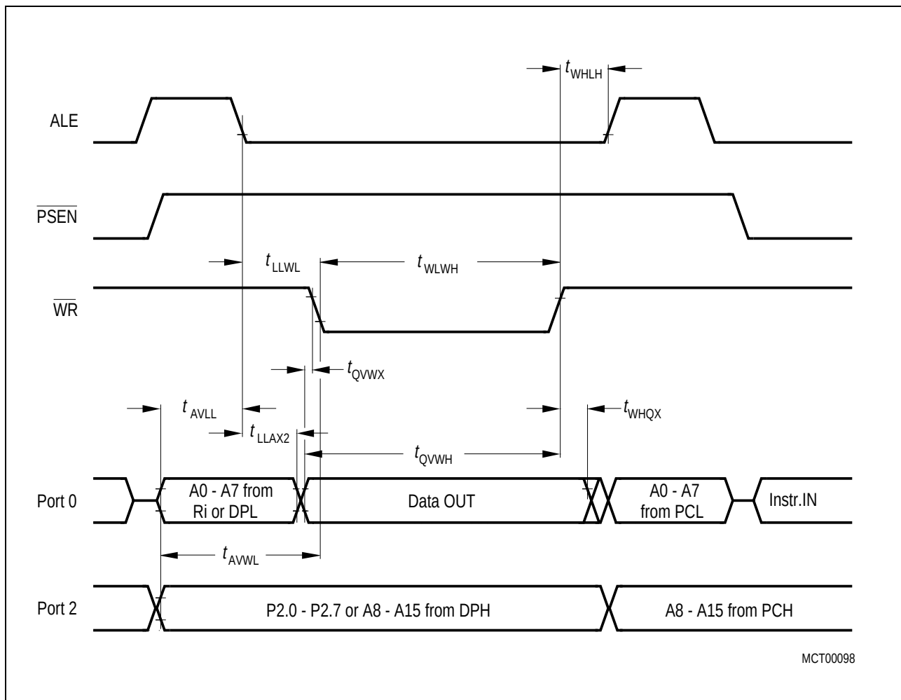
Data Memory Write Cycle
