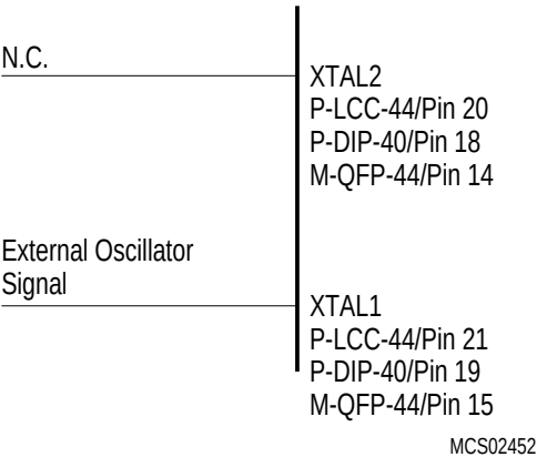
Driving from External Source
