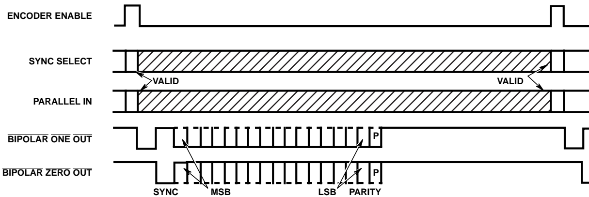
FIGURE 4. ENCODER TIMING
