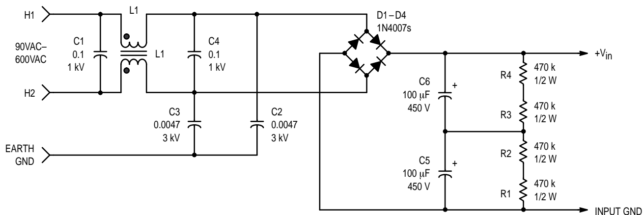
Figure 15. The AC Input/Filter Circuit Section
