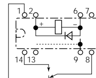
SPDT-1 Form C w/electrostatic shield and diode
