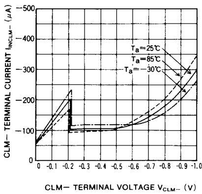
CLM- TERMINAL CURRENT
