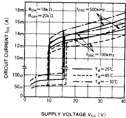
CIRCUIT CURRENT VS. SUPPLY VOLTAGE (NORMAL OPERATION)
