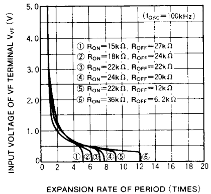
INPUT VOLTAGE OF VF TERMINAL VS. EXPANSION RATE OF PERIOD
