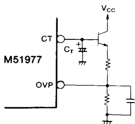
Fig. 39 Application circuit diagram to keep the non-operating condition when over load current condition will continue for specified duration
