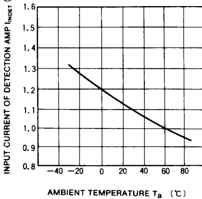
INPUT CURRENT OF DETECTION AMP VS. AMBIENT TEMPERATURE
