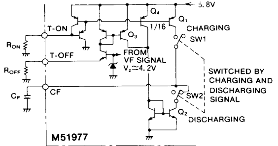
Fig. 4 Schematic diagram of charging and discharging control circuit for OSC. capacitor C F
