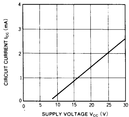
Fig. 23 I_{CC} vs. V_{CC} in OVP operation
