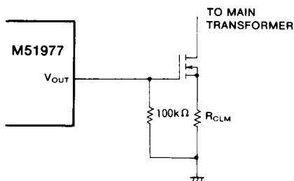
Fig. 40 Circuit diagram to prevent the MOS-FET gate potential rising
