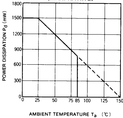
THERMAL DERATING CURVE (MAX. RATING)
