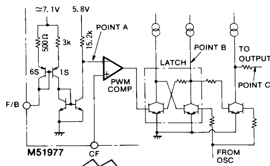
Fig. 9 PWM comparator and latch circuit
