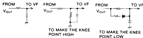
Fig. 36 How to control the knee point
