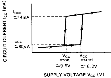
Fig. 3 Circuit current vs. supply voltage
