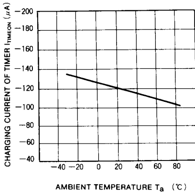
CHARGING CURRENT OF TIMER VS. AMBIENT TEMPERATURE
