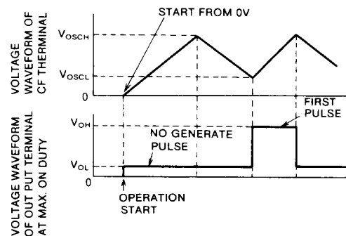
Fig. 7 Relation between OSC. and output waveform circuit operation at start up
