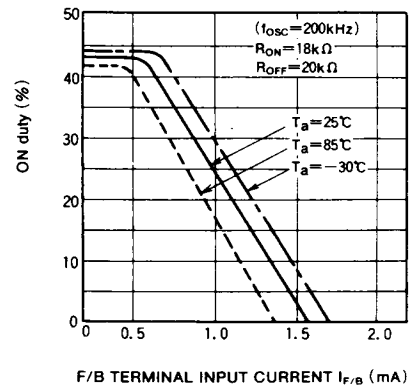
ON duty VS. F/B TERMINAL INPUT CURRENT
