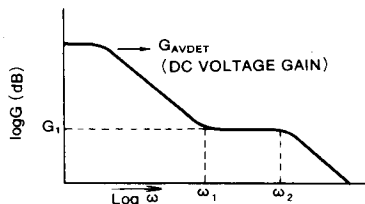
Fig. 44 Gain-frequency characteristics between point B and C shown in Fig. 43
