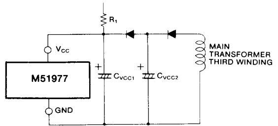
Fig. 27 DC source circuit for stable start-up
