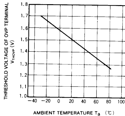
THRESHOLD VOLTAGE OF OVP TERMINAL VS. AMBIENT TEMPERATURE
