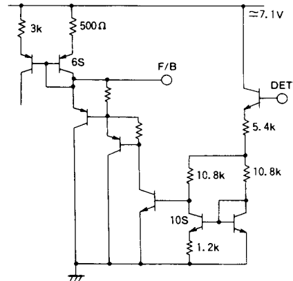
Fig. 17 Equivalent circuit diagram of voltage detector
