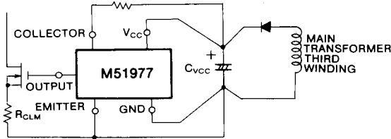
Fig. 26 How to design the conductor-pattern of type M51977 on PC board (schematic example)
