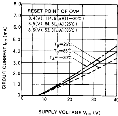
CIRCUIT CURRENT VS. SUPPLY VOLTAGE (OVP STATE)
