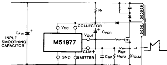
Fig. 31 Peripheral circuit diagram of CLM+ terminal
