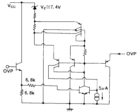
Fig. 22 Equivalent circuit diagram of OVP
