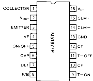
Outline 16P4
