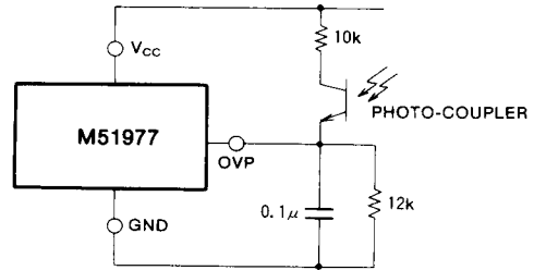
Fig. 28 Peripheral circuit of OVP terminal
