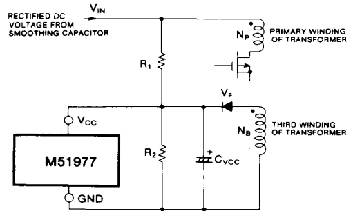
Fig. 25 Start-up circuit diagram when it is necessary to set the start and stop input voltage
