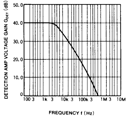
DETECTION AMP VOLTAGE GAIN VS. FREQUENCY
