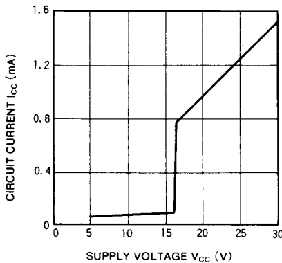
Fig. 21 I_{CC} vs. V_{CC} in OFF state
