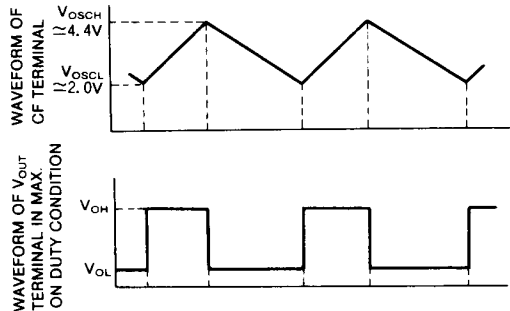
Fig. 5 OSC. waveform at normal condition (no-operation of intermittent action and OSC. control circuit)
