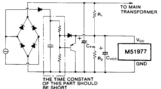
Fig. 29 Example circuit diagram to make the OVP-reset-time fast
