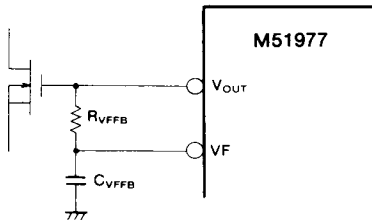
Fig. 35 Feed back loop through low pass filter from V_{OUT} to VF terminal
