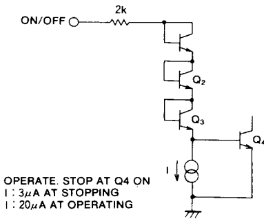
Fig. 19 ON/OFF circuit
