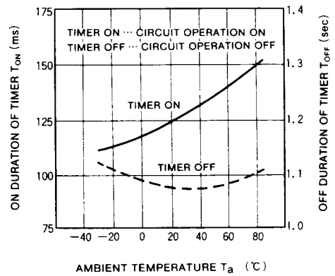
ON AND OFF DURATION OF TIMER VS. AMBIENT TEMPERATURE (INTERMITTENT OPERATION)
