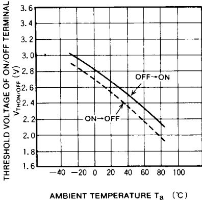
THRESHOLD VOLTAGE OF ON/OFF TERMINAL VS. AMBIENT TEMPERATURE
