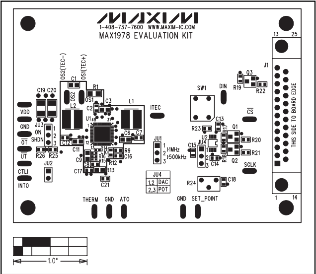
Figure 6. MAX1978 EV Kit Component Placement Guide—Component Side
