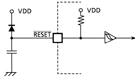
Figure 2-23. Simplified Power-On-Reset
