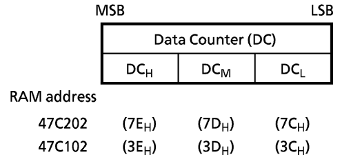
Figure 2-7. Data Counter
