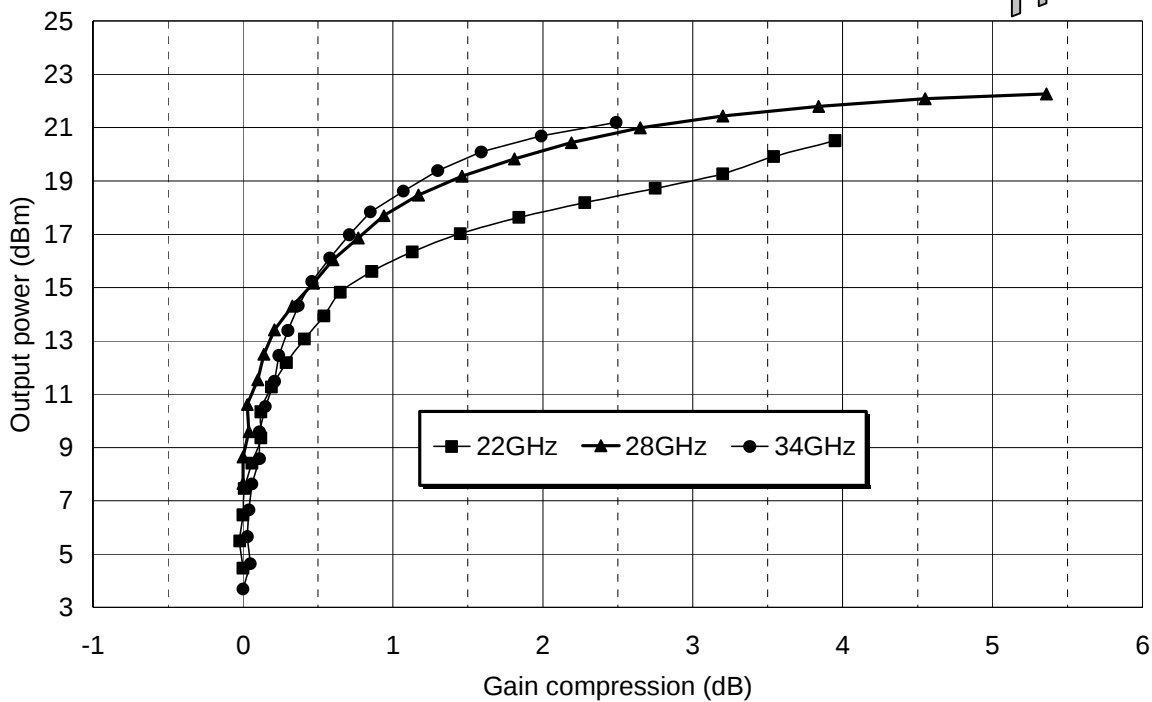
Output Power versus Gain Compression
