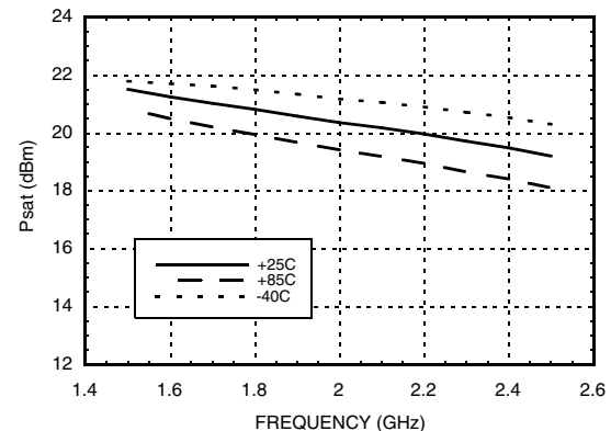
Output Psat*
